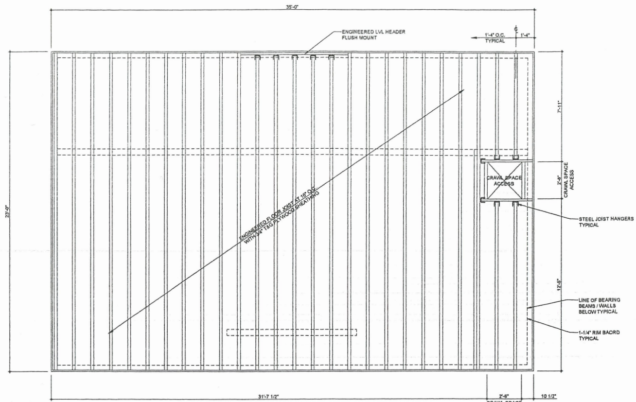
FIRST FLOOR FRAMING PLAN 1/4" = 1'-0"
