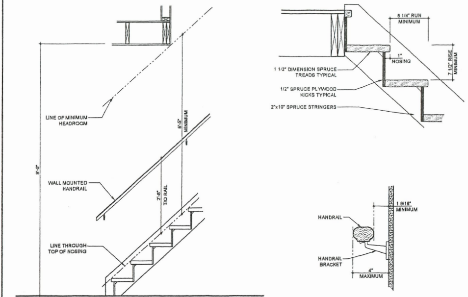
TYPICAL INTERIOR STAIR DETAILS NTS
