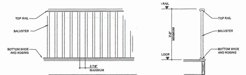
TYPICAL INTERIOR STAIR DETAILS NTS
