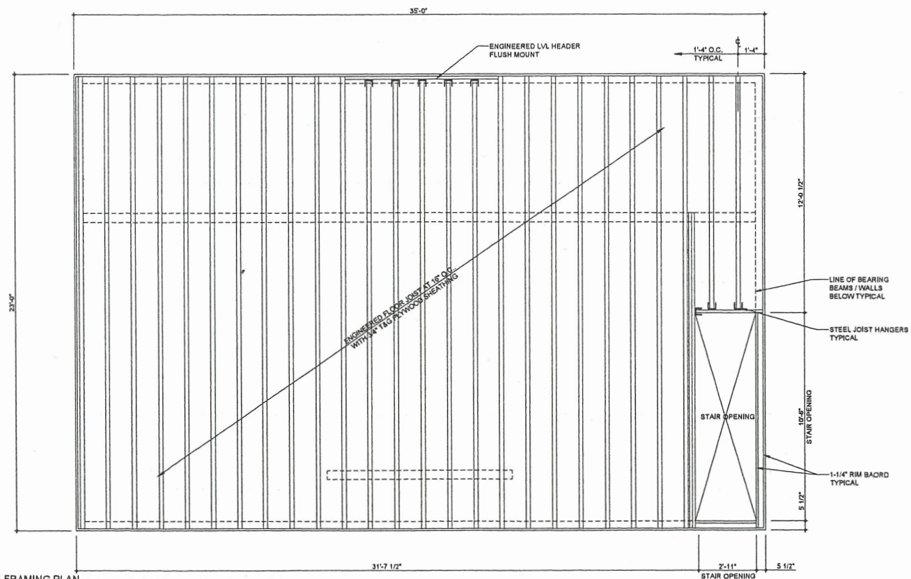
SECOND FLOOR FRAMING PLAN 1/4" = 1'-0"
