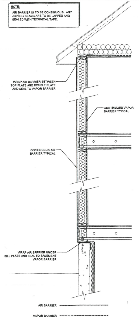
TYPICAL AIR BARRIER / VAPOR BARRIER 1" = 1/2'-0"
